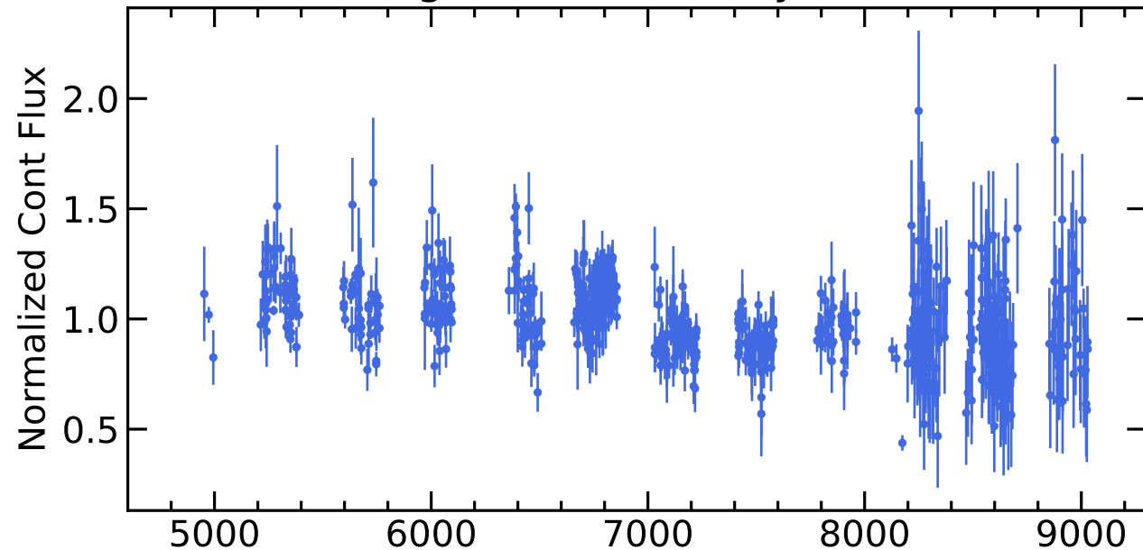
RM270 Light Curves (w/ PyROA model)
