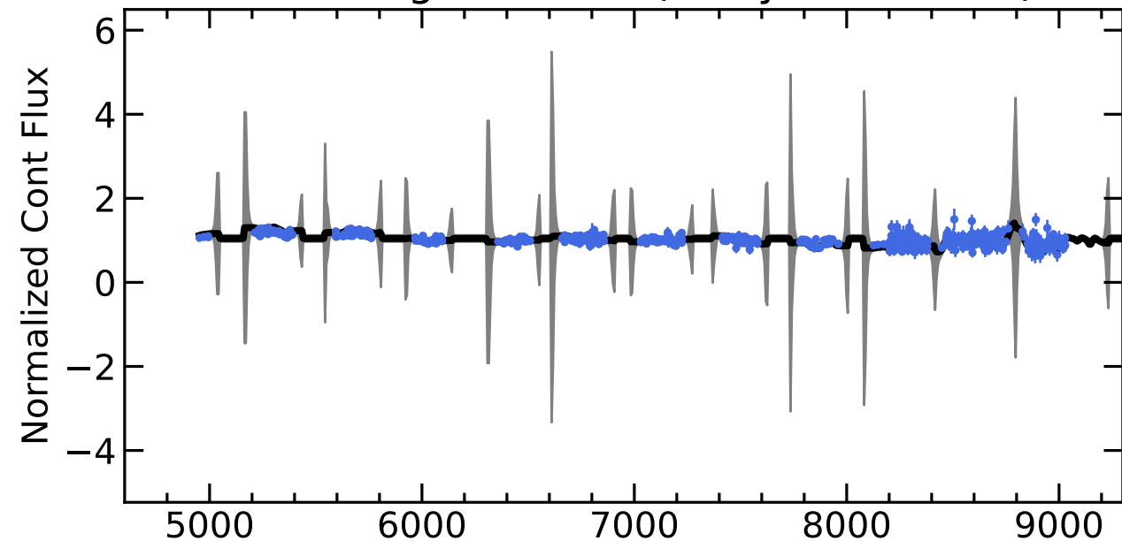
RM271 Light Curves (w/ PyROA model)
