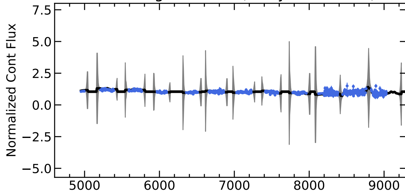
RM271 Light Curves (w/ PyROA model)
