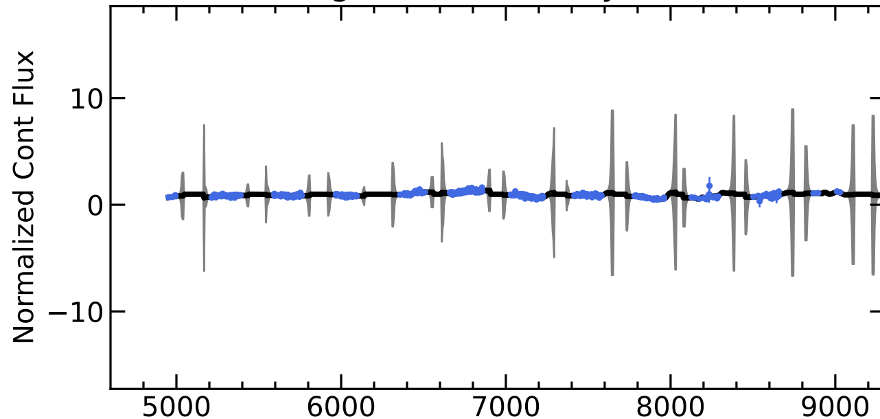
RM274 Light Curves (w/ PyROA model)
