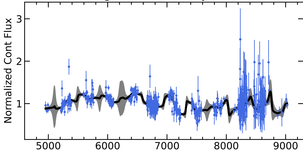
RM277 Light Curves (w/ PyROA model)
