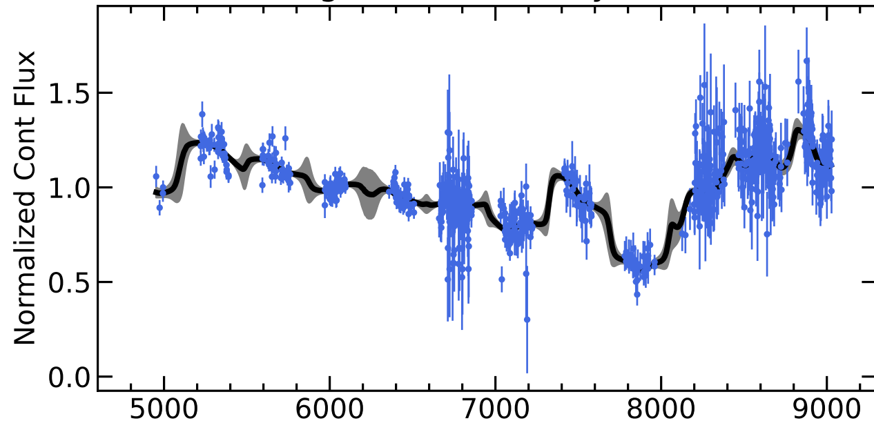
RM278 Light Curves (w/ PyROA model)
