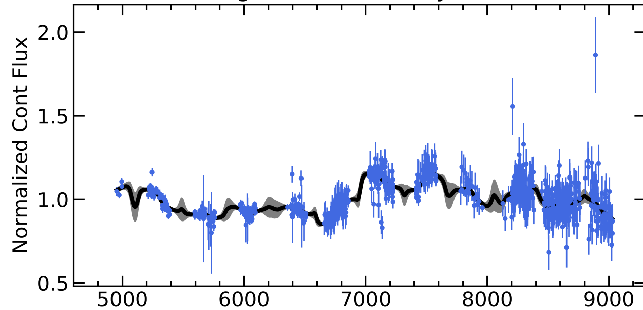
RM280 Light Curves (w/ PyROA model)
