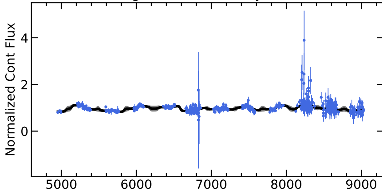
RM281 Light Curves (w/ PyROA model)
