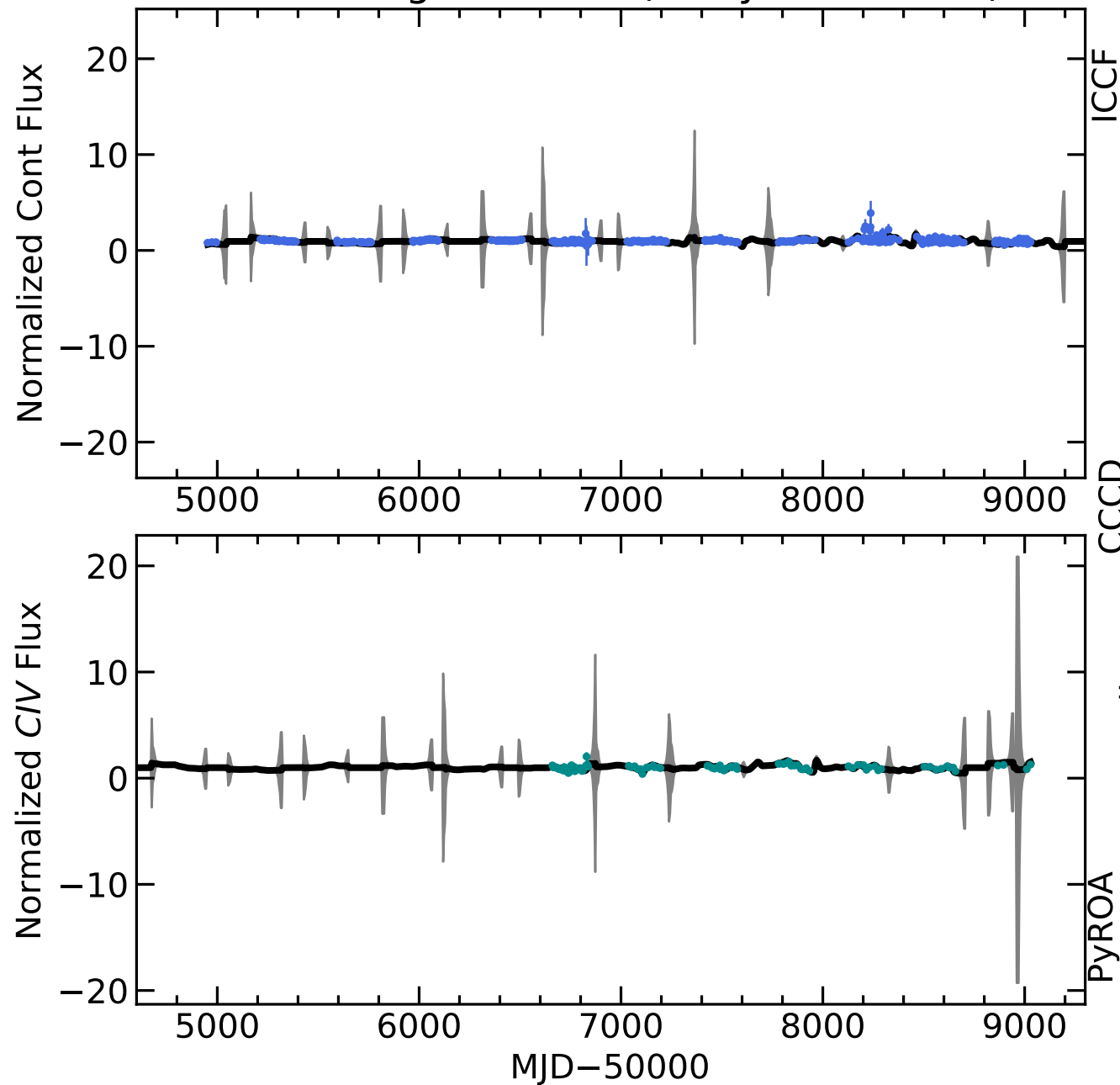
RM281 Light Curves (w/ PyROA model)
