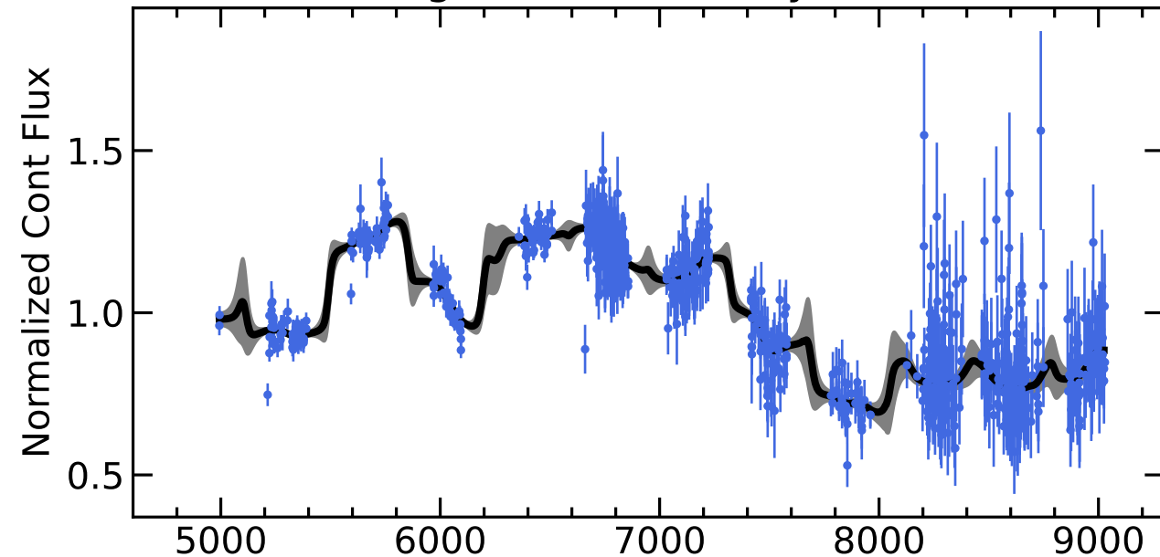
RM283 Light Curves (w/ PyROA model)
