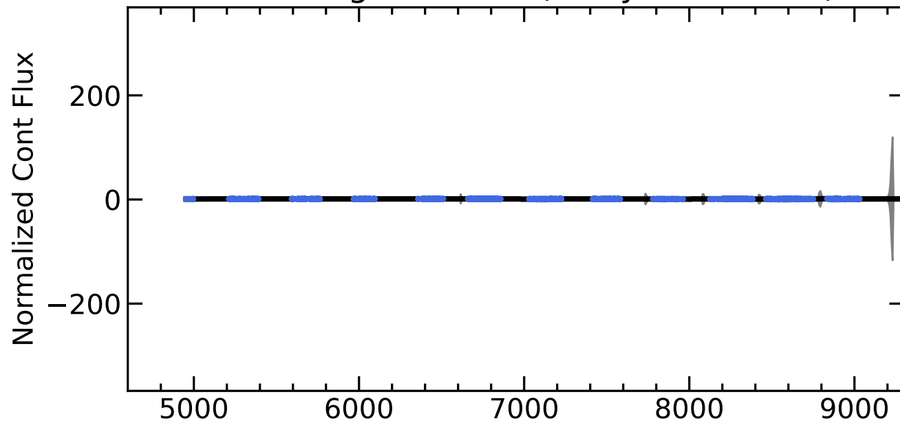
RM284 Light Curves (w/ PyROA model)
