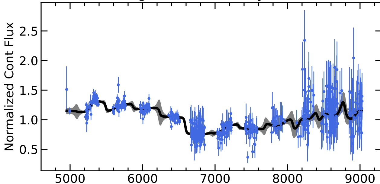
RM286 Light Curves (w/ PyROA model)
