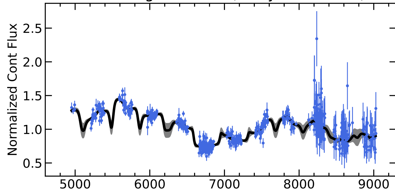
RM288 Light Curves (w/ PyROA model)
