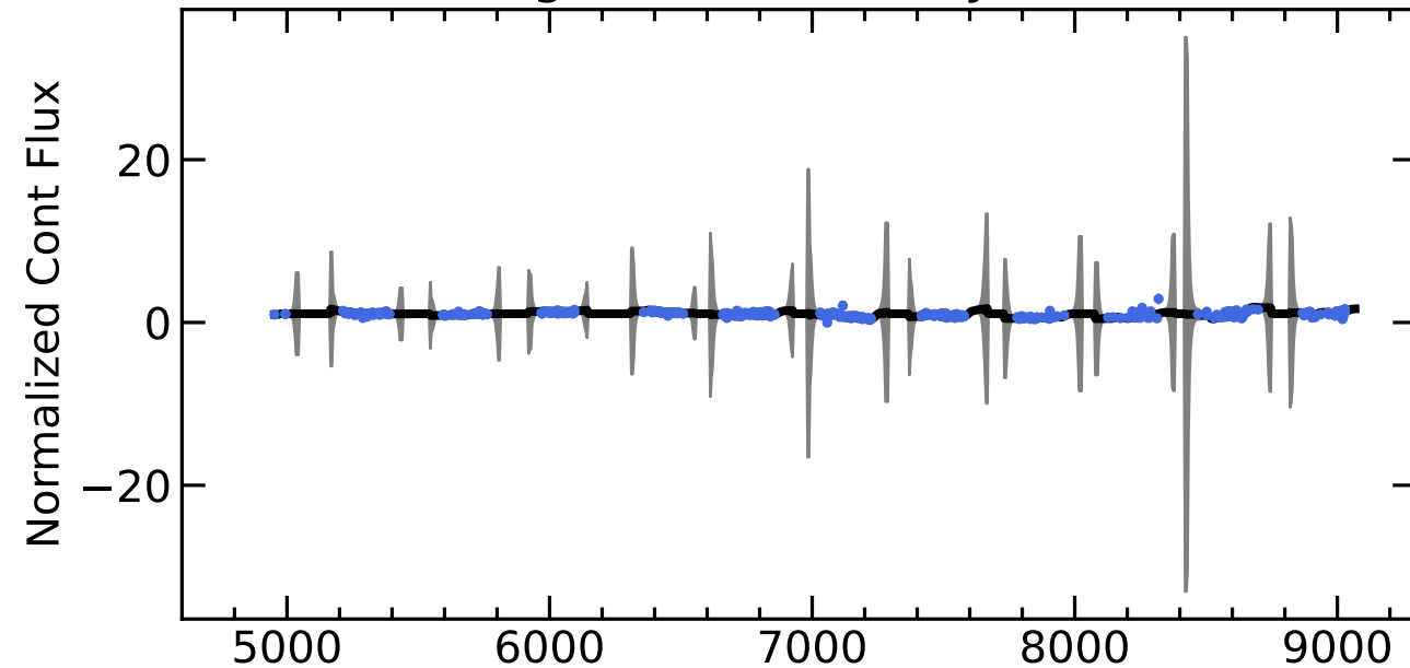
RM289 Light Curves (w/ PyROA model)
