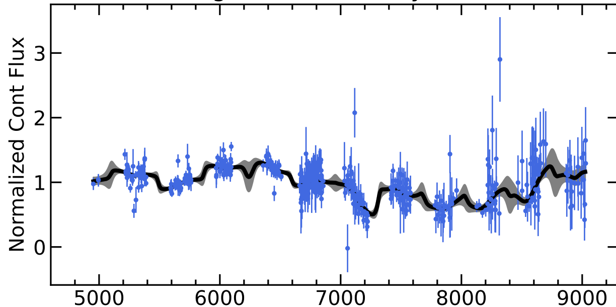
RM289 Light Curves (w/ PyROA model)
