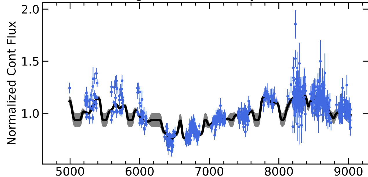
RM290 Light Curves (w/ PyROA model)
