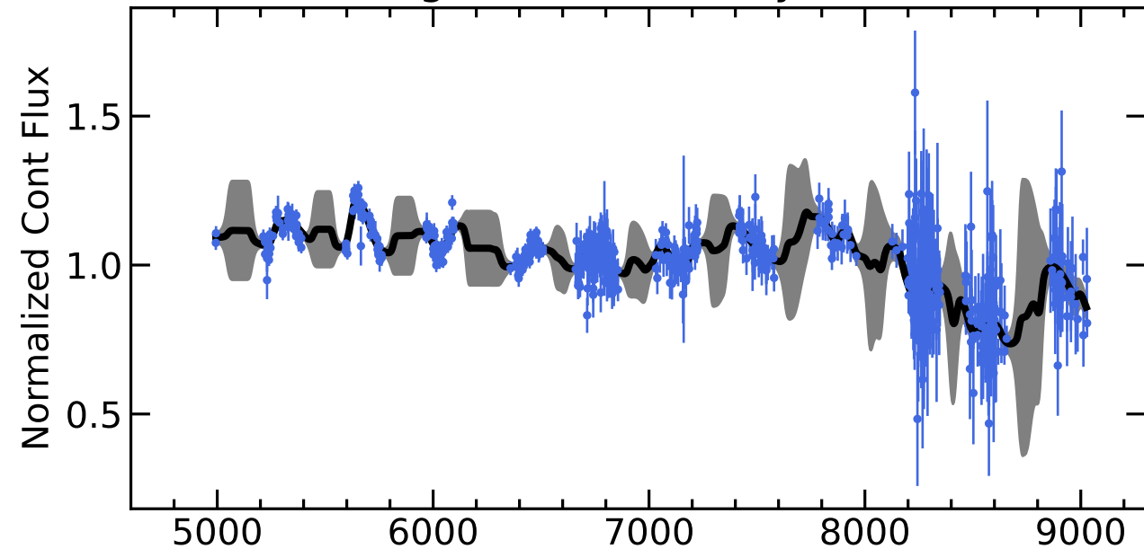
RM292 Light Curves (w/ PyROA model)
