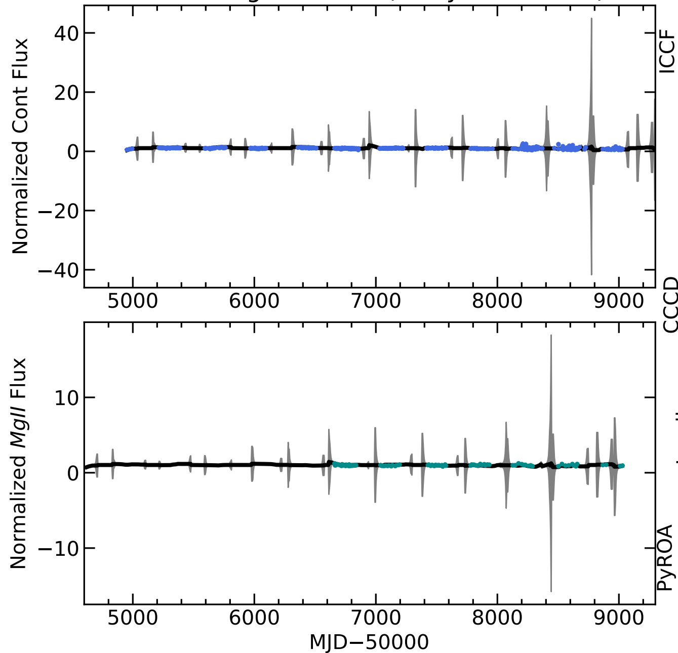
RM293 Light Curves (w/ PyROA model)
