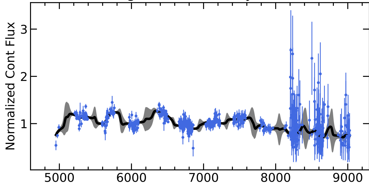
RM293 Light Curves (w/ PyROA model)
