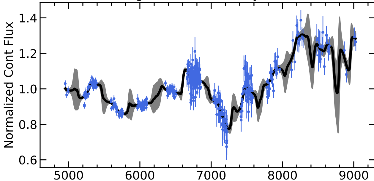
RM294 Light Curves (w/ PyROA model)
