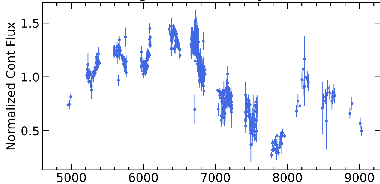
RM295 Light Curves (w/ PyROA model)
