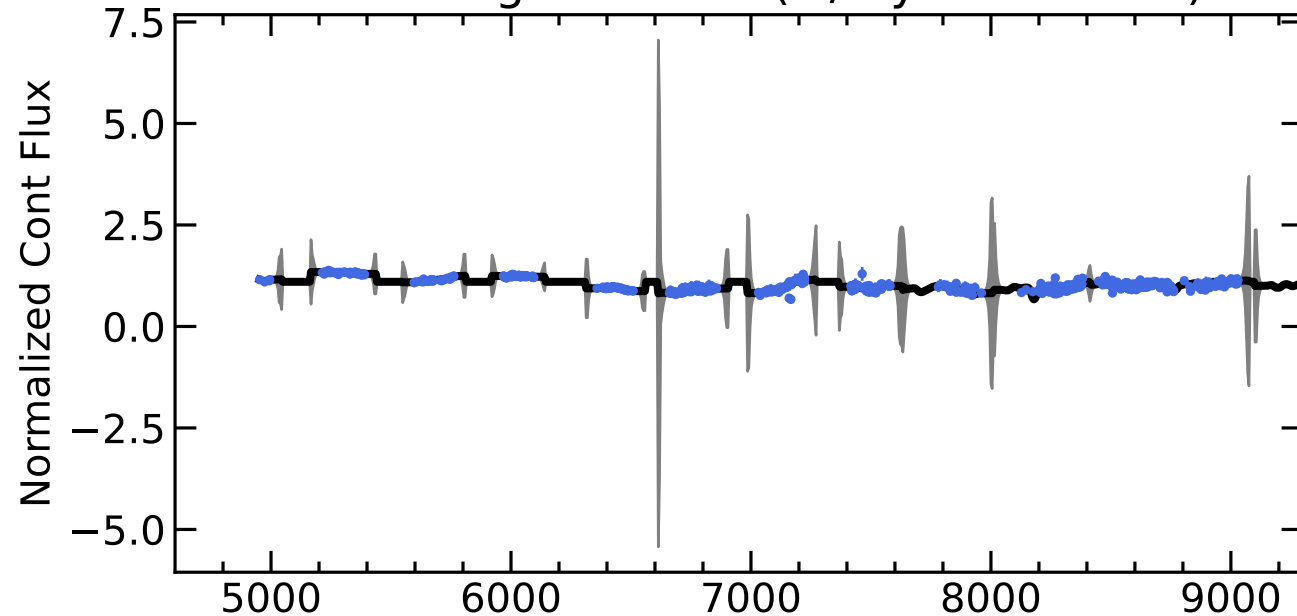
RM296 Light Curves (w/ PyROA model)
