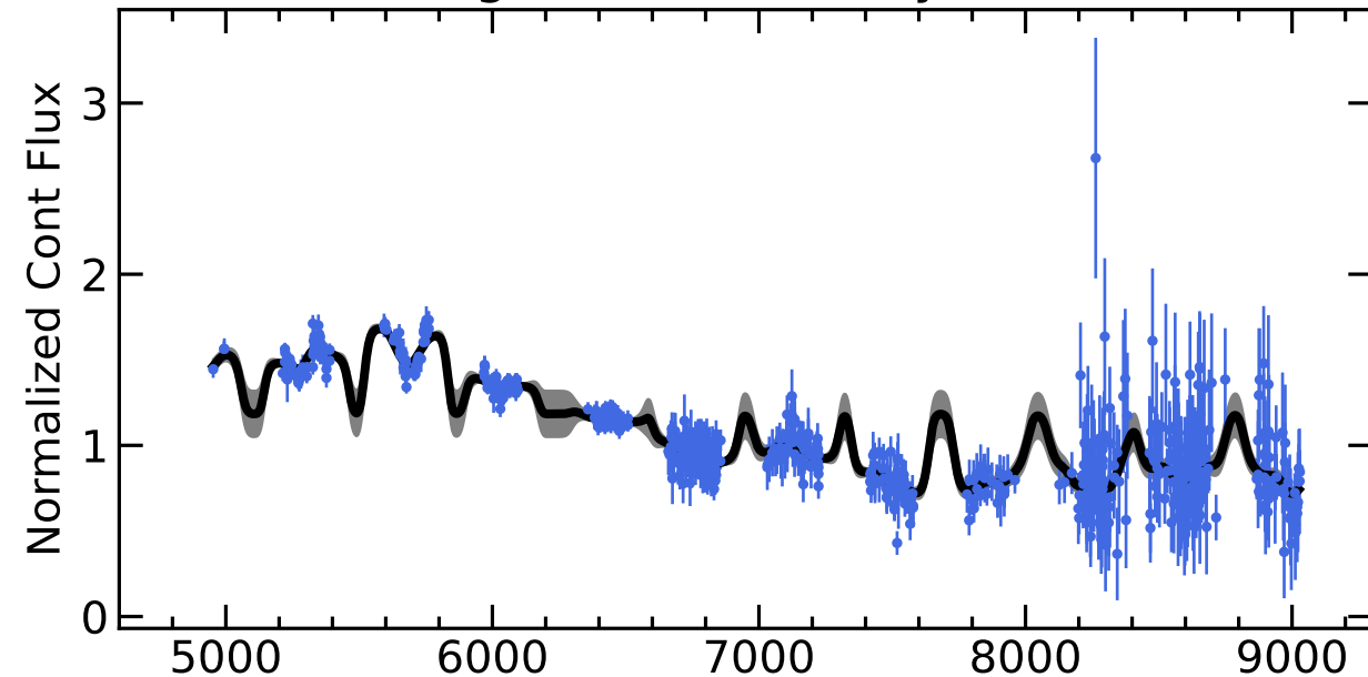
RM297 Light Curves (w/ PyROA model)
