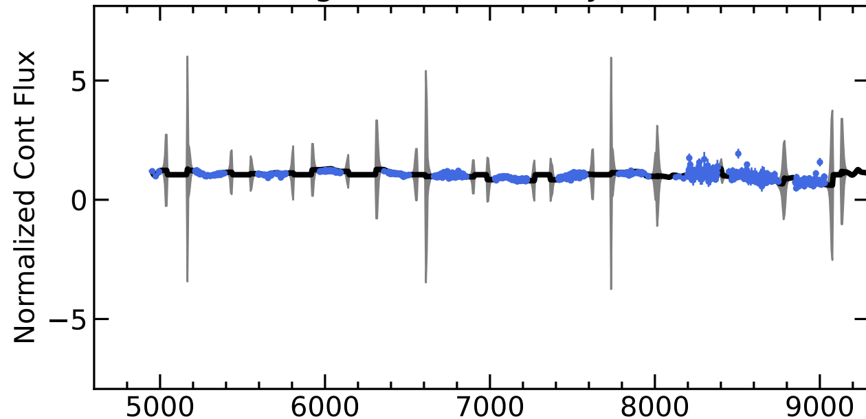
RM298 Light Curves (w/ PyROA model)
