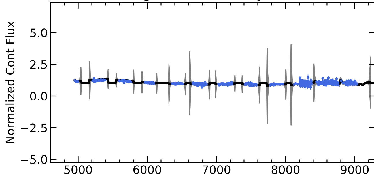
RM299 Light Curves (w/ PyROA model)
