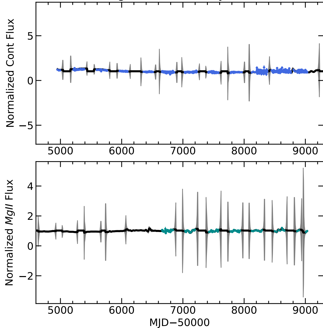
RM299 Light Curves (w/ PyROA model)
