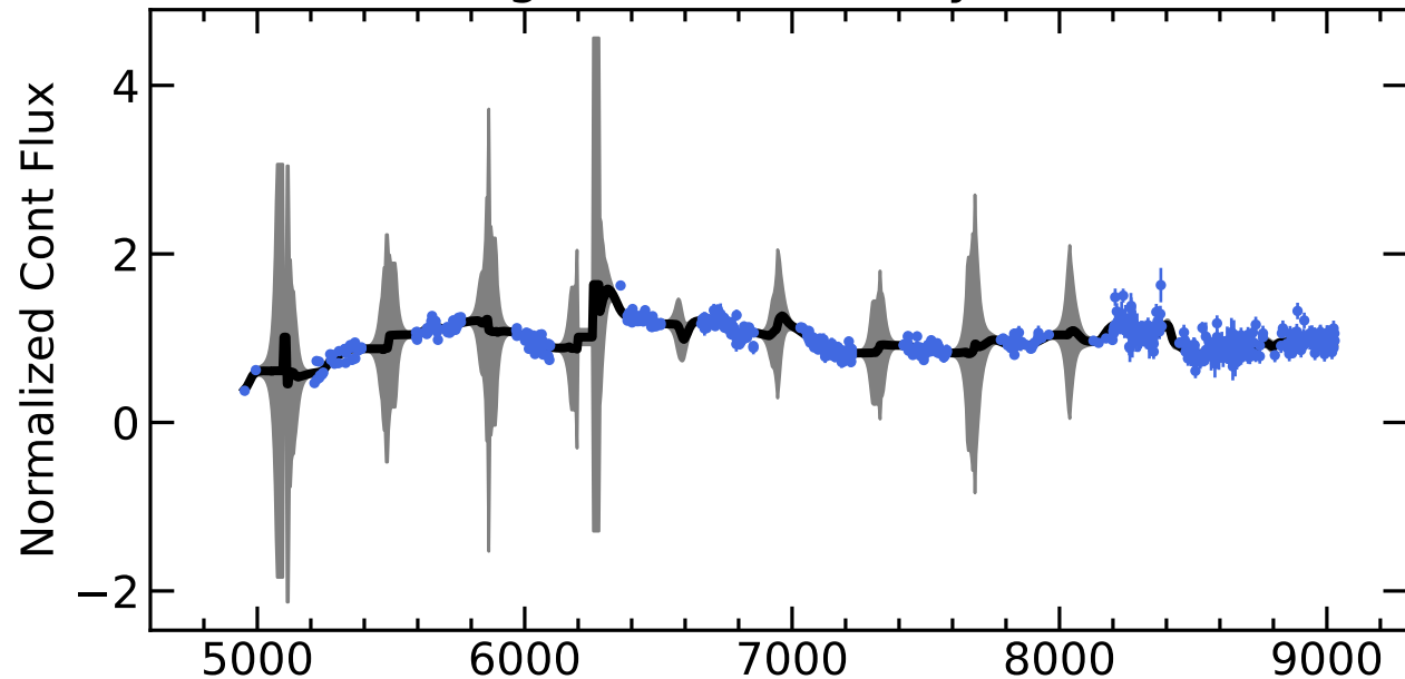
RM300 Light Curves (w/ PyROA model)
