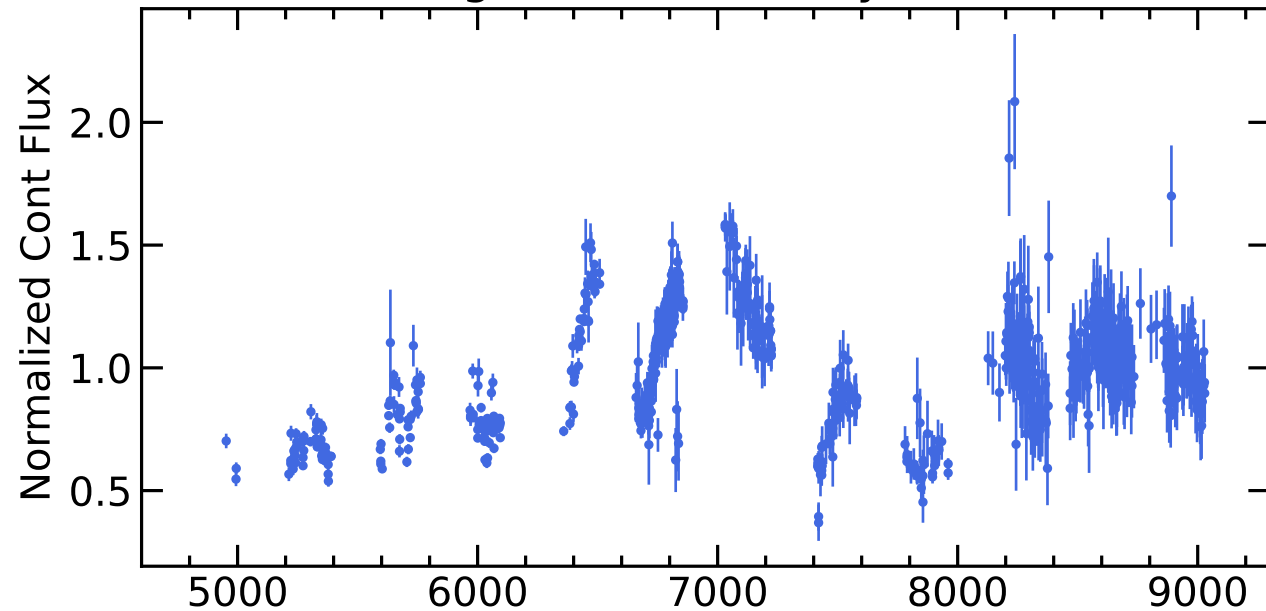
RM301 Light Curves (w/ PyROA model)
