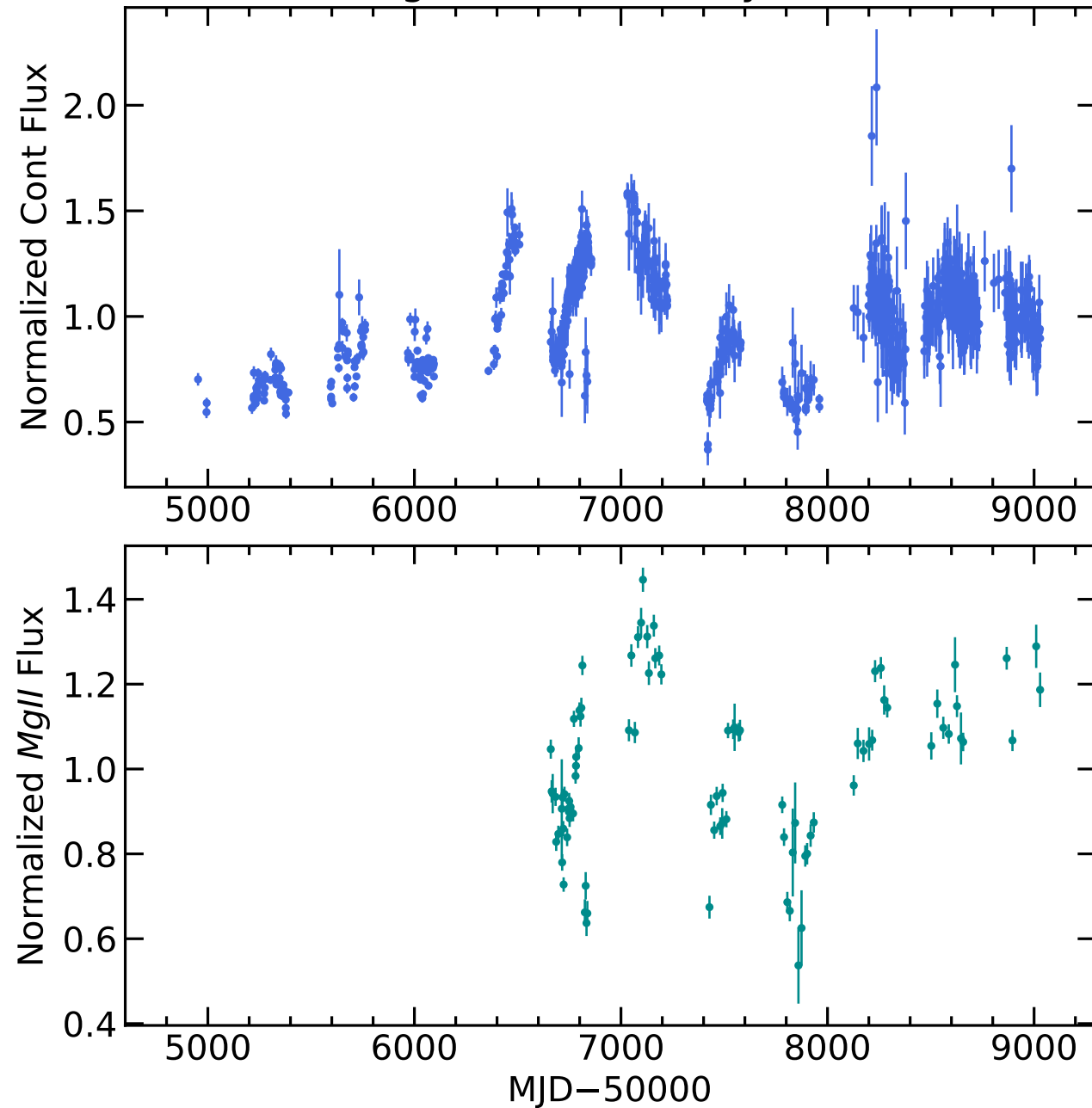
RM301 Light Curves (w/ PyROA model)
