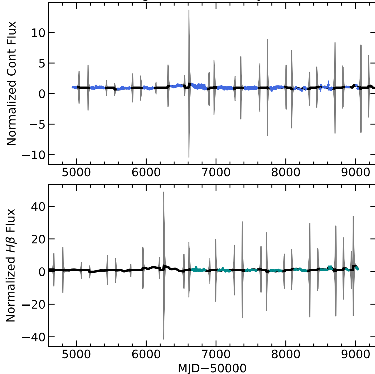
RM302 Light Curves (w/ PyROA model)
