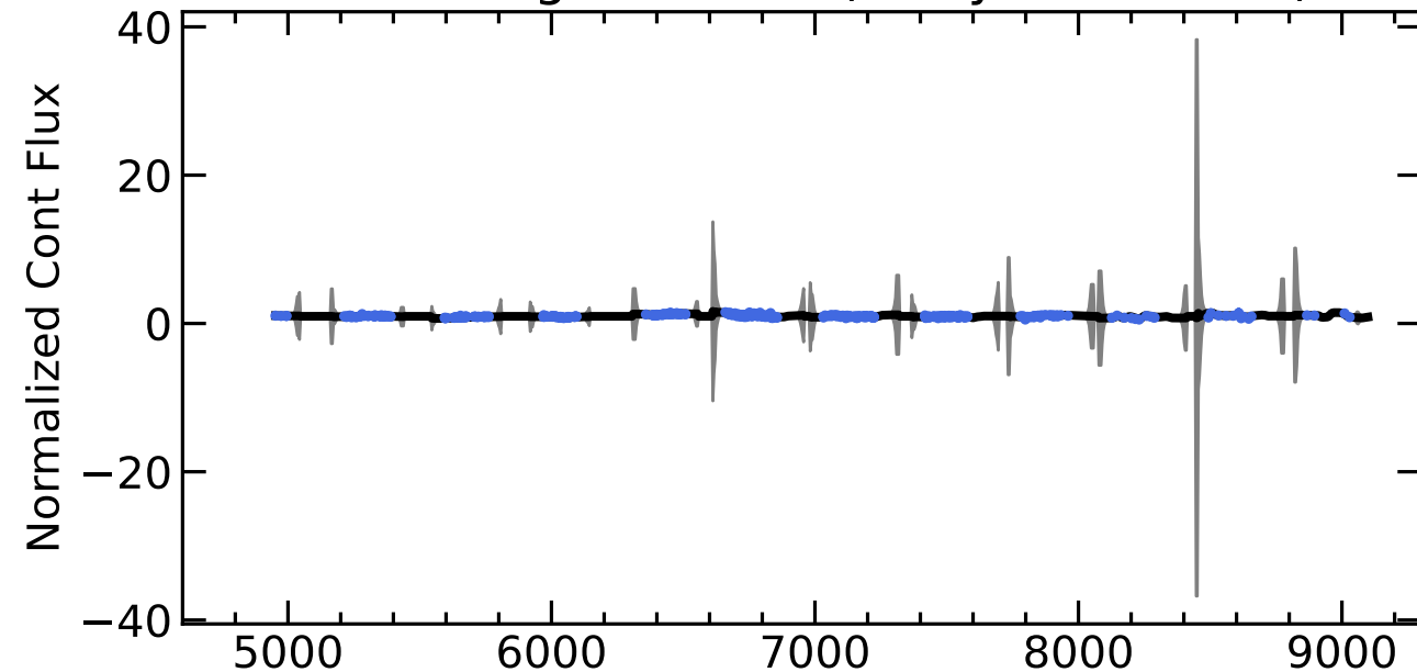
RM302 Light Curves (w/ PyROA model)
