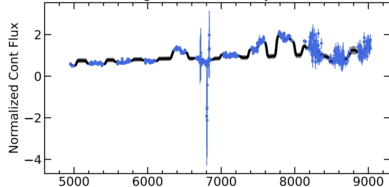
RM303 Light Curves (w/ PyROA model)
