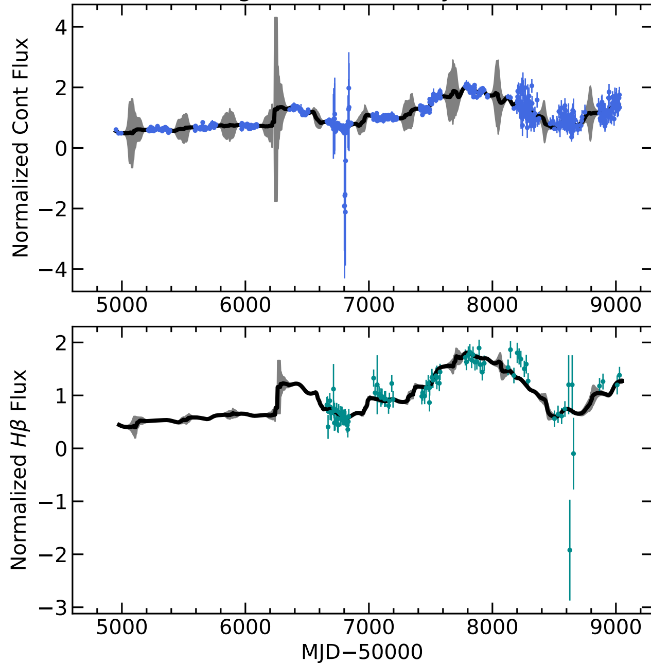
RM303 Light Curves (w/ PyROA model)
