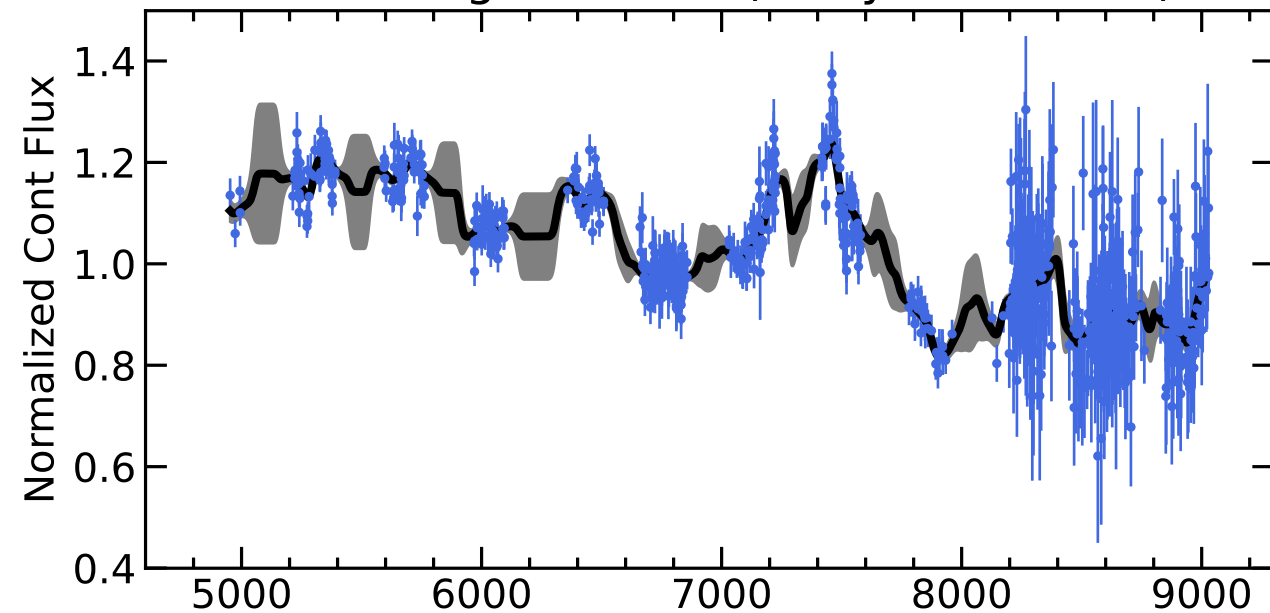
RM305 Light Curves (w/ PyROA model)
