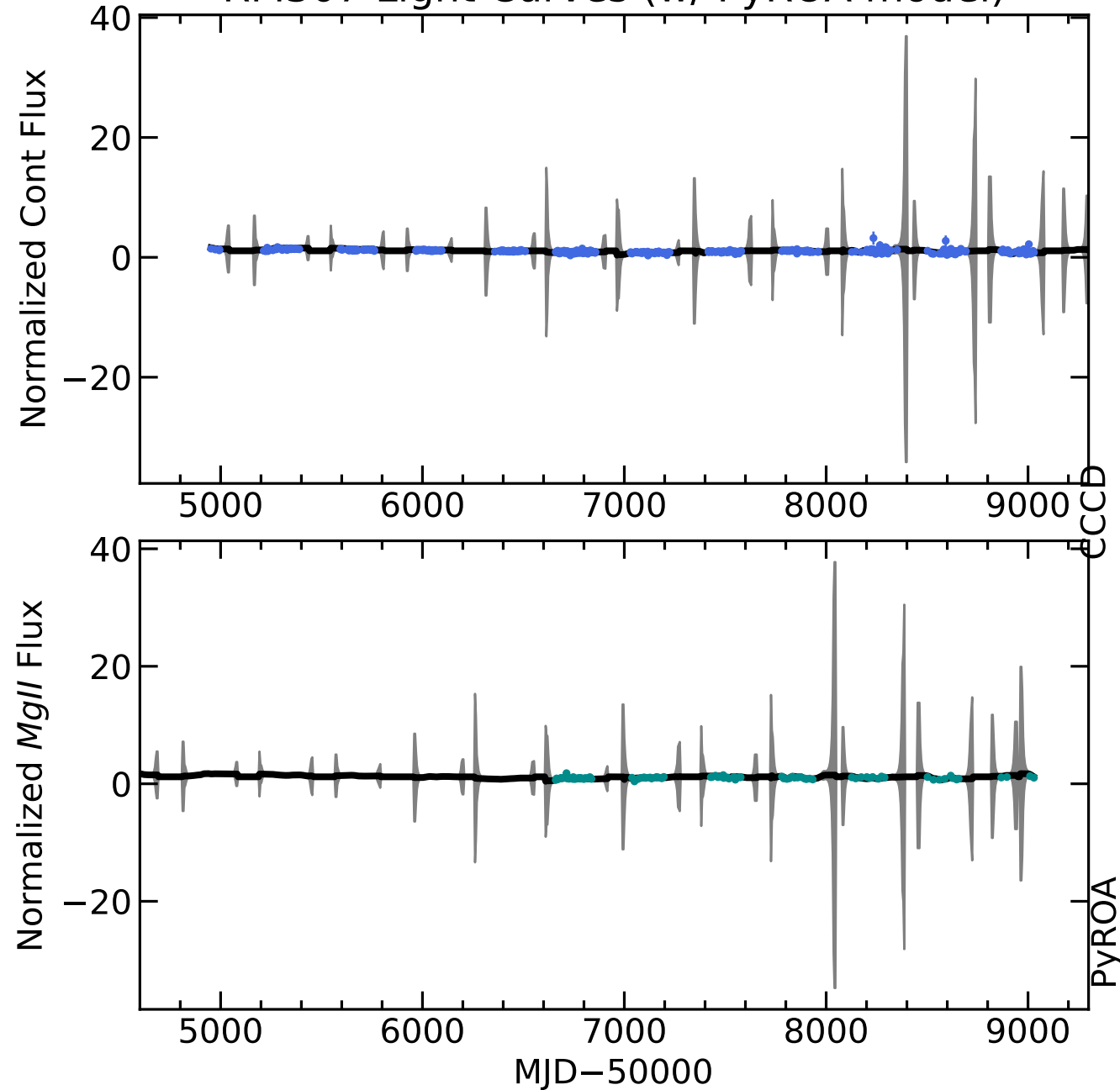
RM307 Light Curves (w/ PyROA model)
