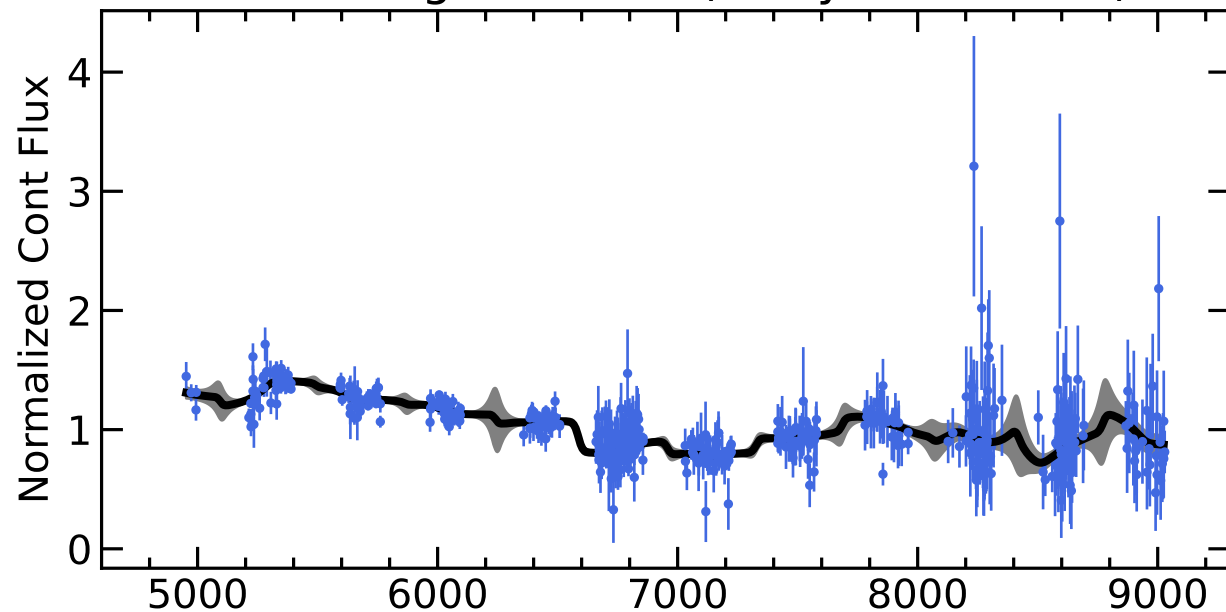
RM307 Light Curves (w/ PyROA model)
