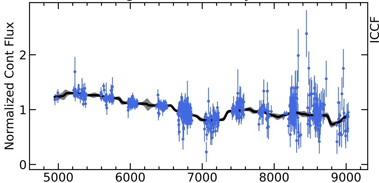
RM308 Light Curves (w/ PyROA model)
