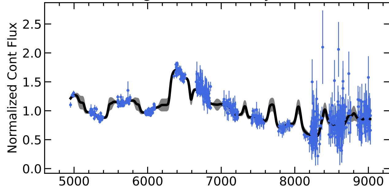
RM309 Light Curves (w/ PyROA model)
