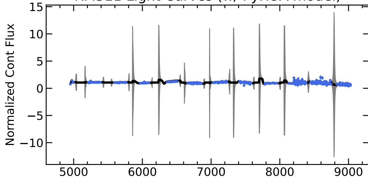
RM311 Light Curves (w/ PyROA model)
