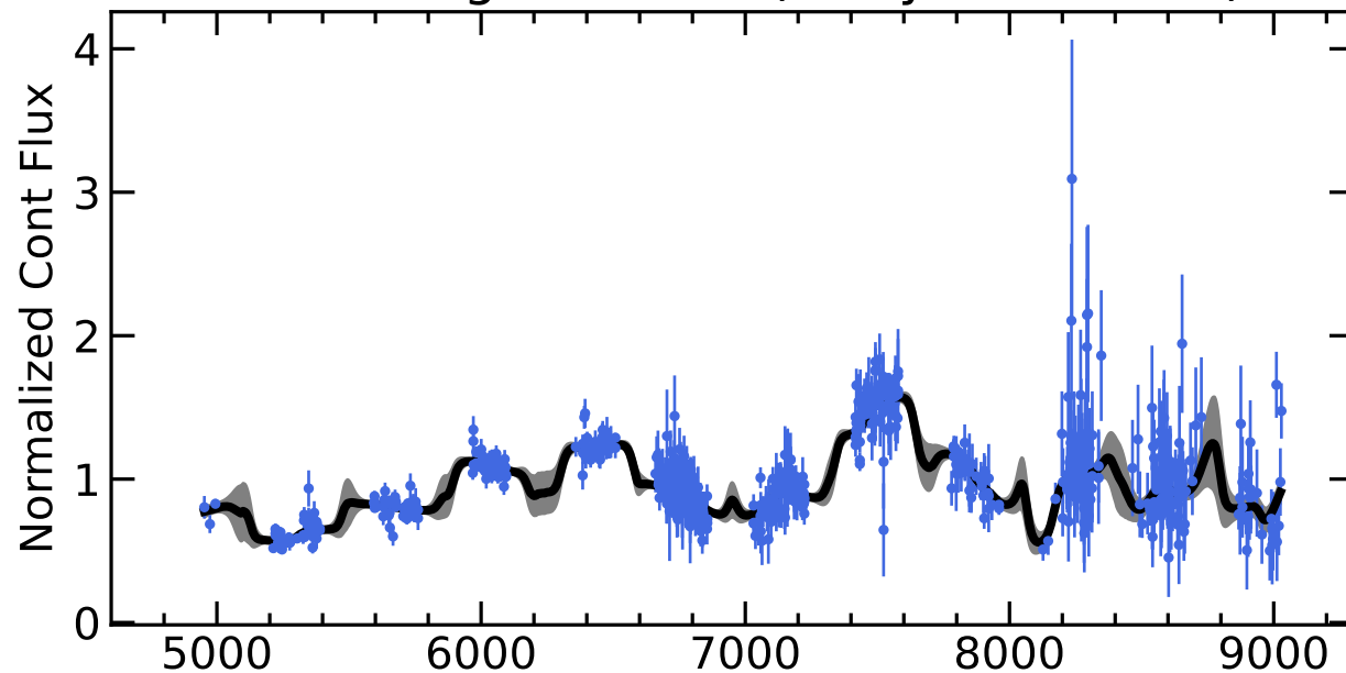
RM312 Light Curves (w/ PyROA model)
