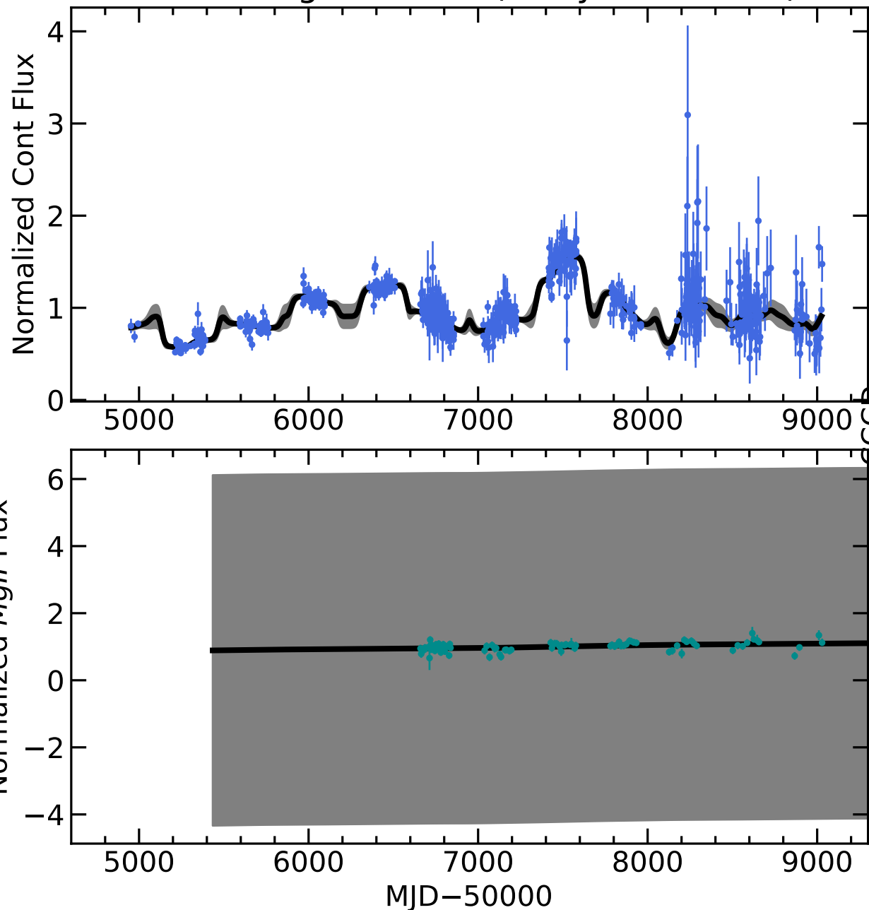
RM312 Light Curves (w/ PyROA model)
