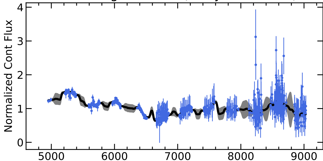
RM313 Light Curves (w/ PyROA model)
