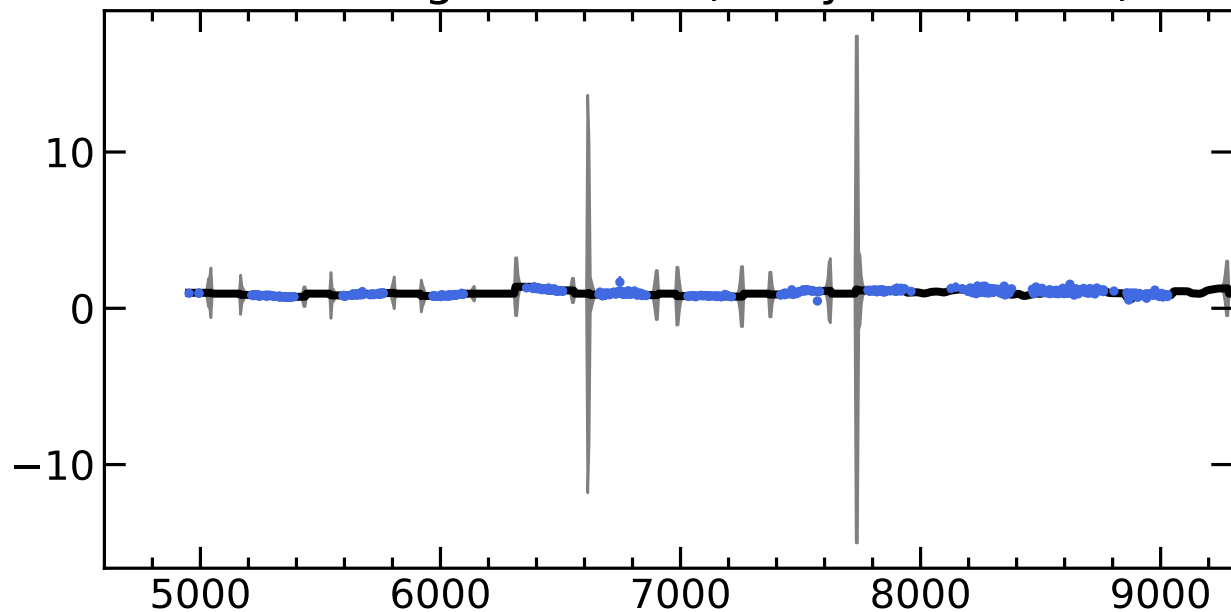
RM317 Light Curves (w/ PyROA model)
