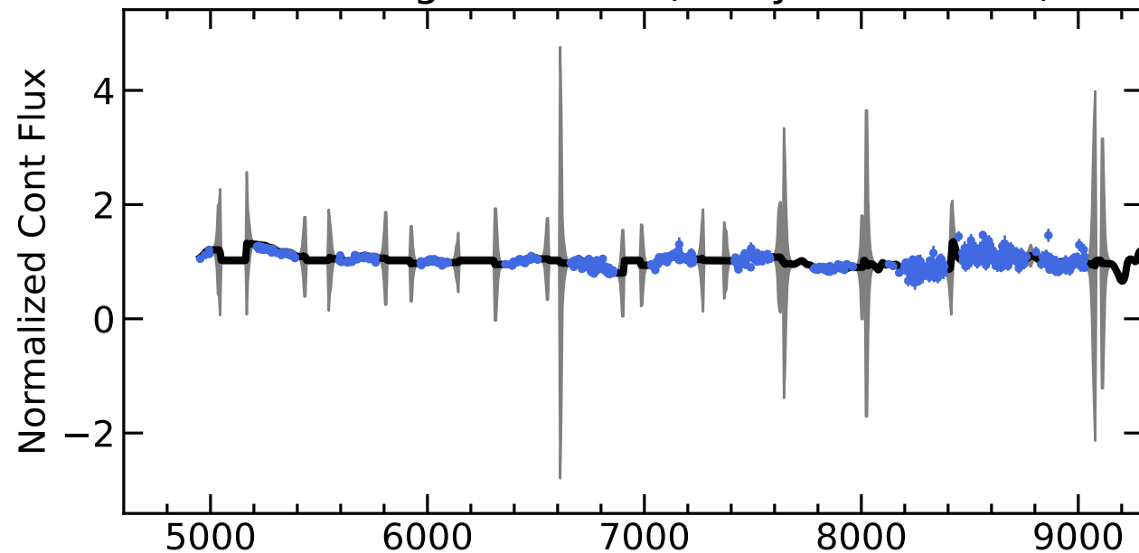
RM318 Light Curves (w/ PyROA model)
