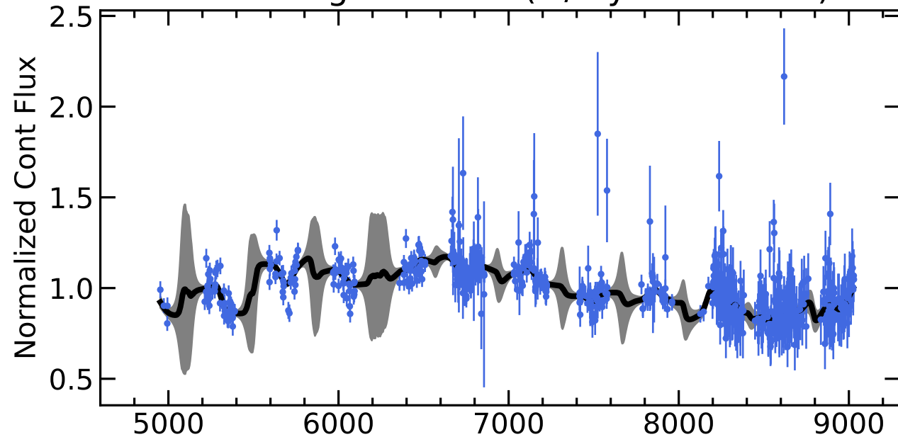
RM320 Light Curves (w/ PyROA model)
