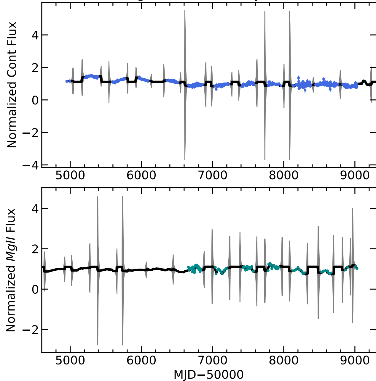
RM321 Light Curves (w/ PyROA model)
