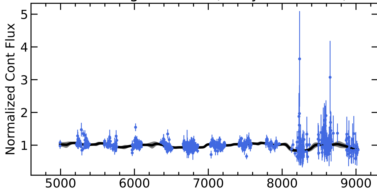
RM323 Light Curves (w/ PyROA model)
