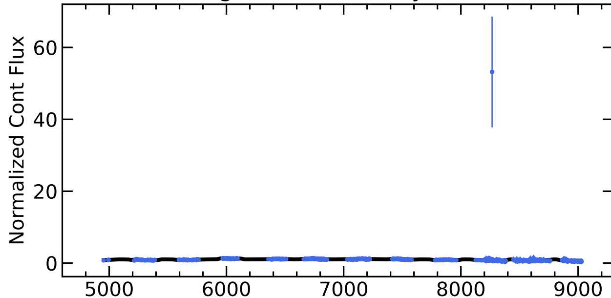
RM324 Light Curves (w/ PyROA model)
