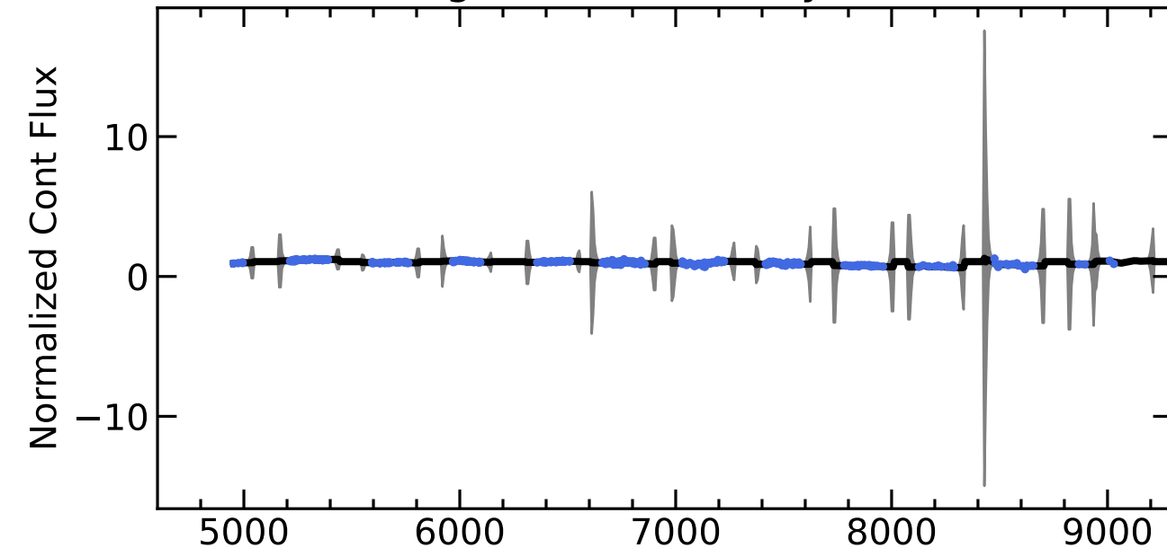
RM325 Light Curves (w/ PyROA model)
