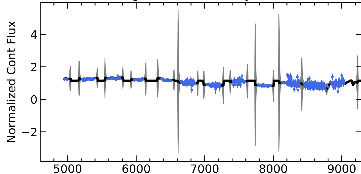
RM327 Light Curves (w/ PyROA model)
