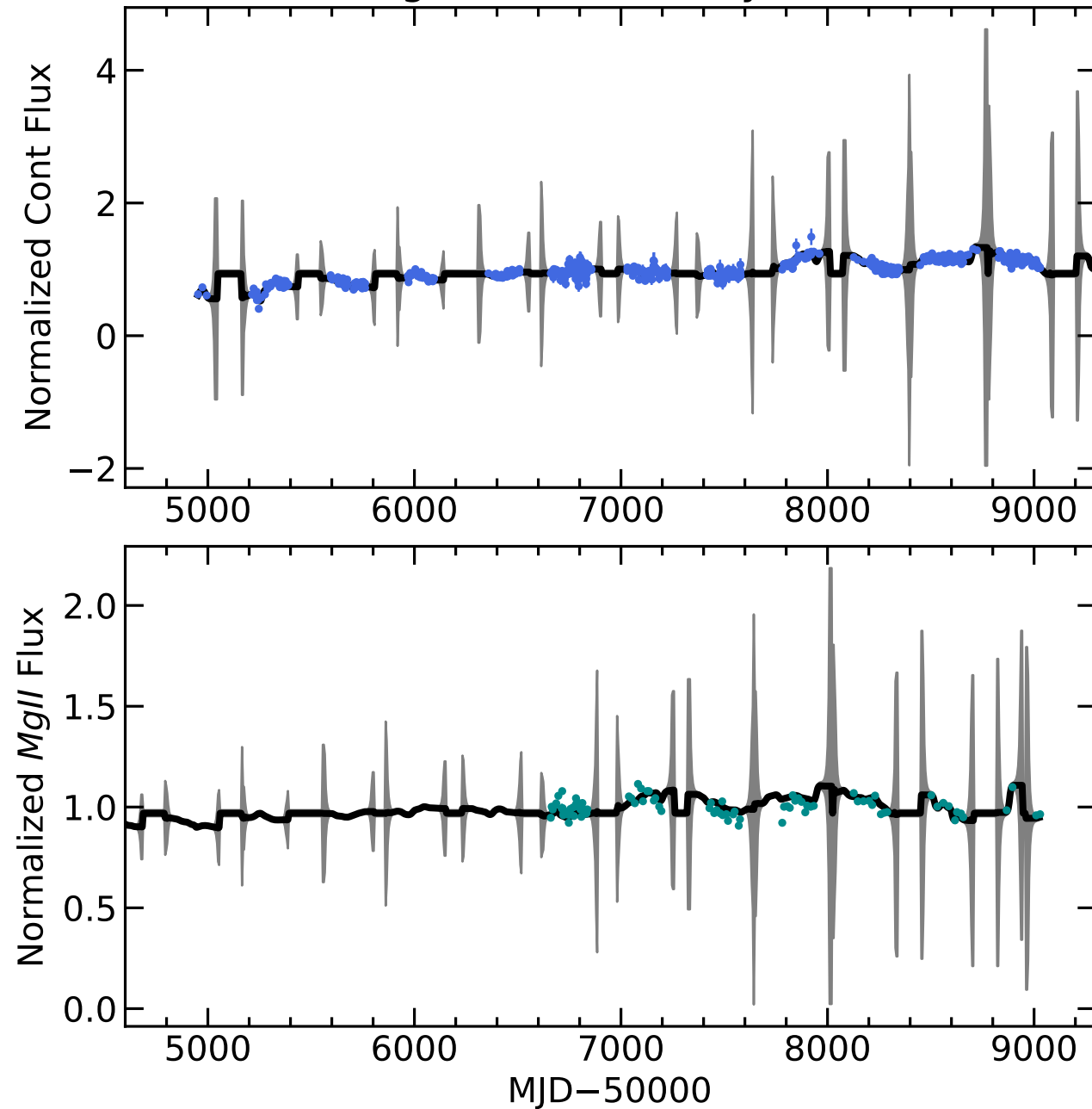
RM329 Light Curves (w/ PyROA model)
