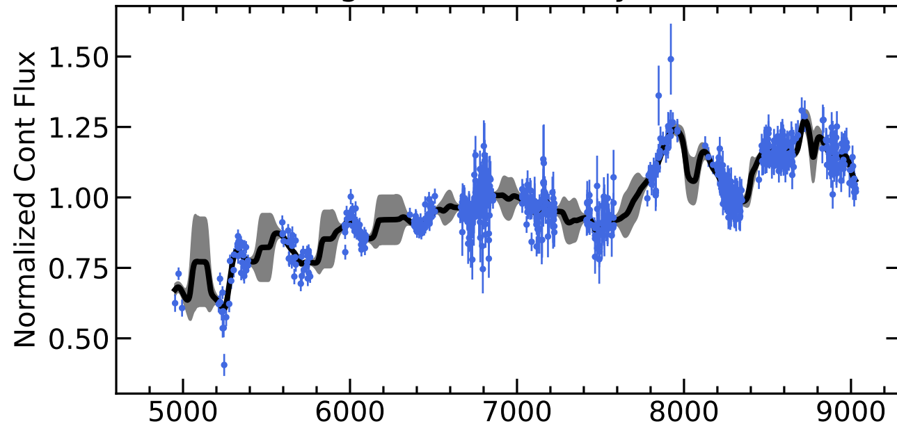
RM329 Light Curves (w/ PyROA model)
