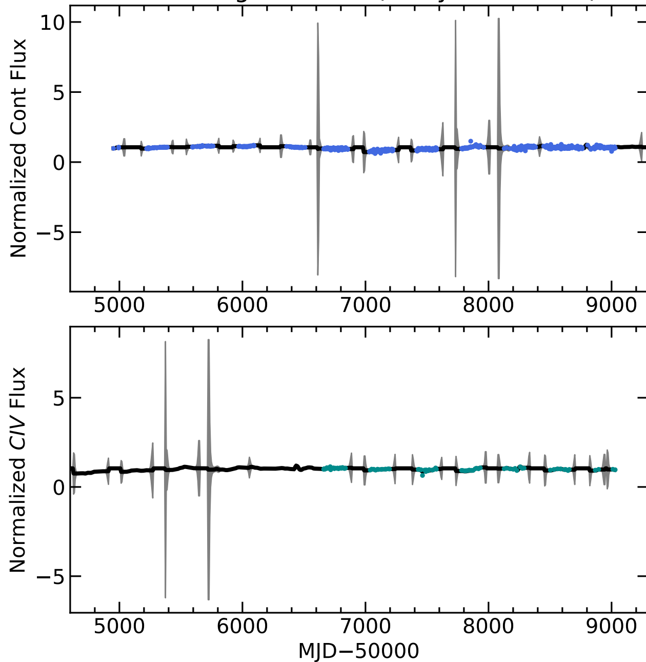
RM330 Light Curves (w/ PyROA model)
