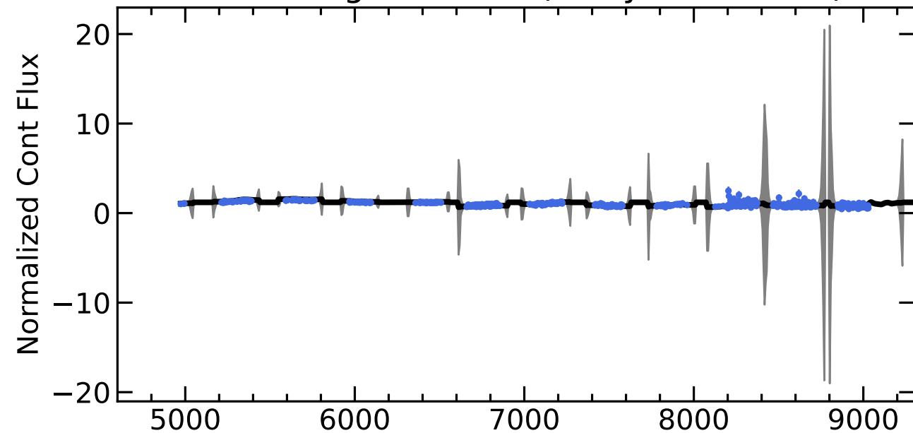
RM332 Light Curves (w/ PyROA model)
