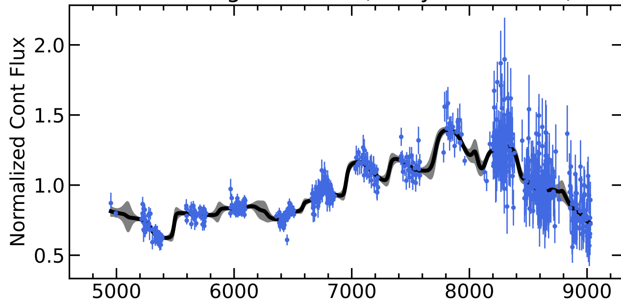
RM334 Light Curves (w/ PyROA model)
