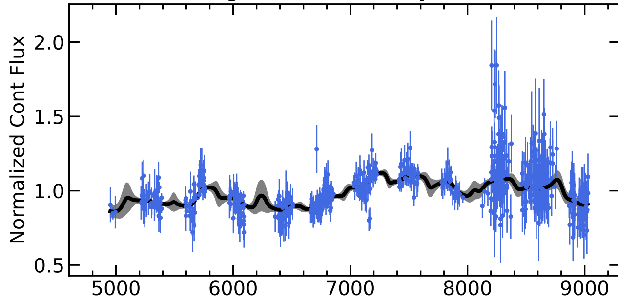
RM335 Light Curves (w/ PyROA model)
