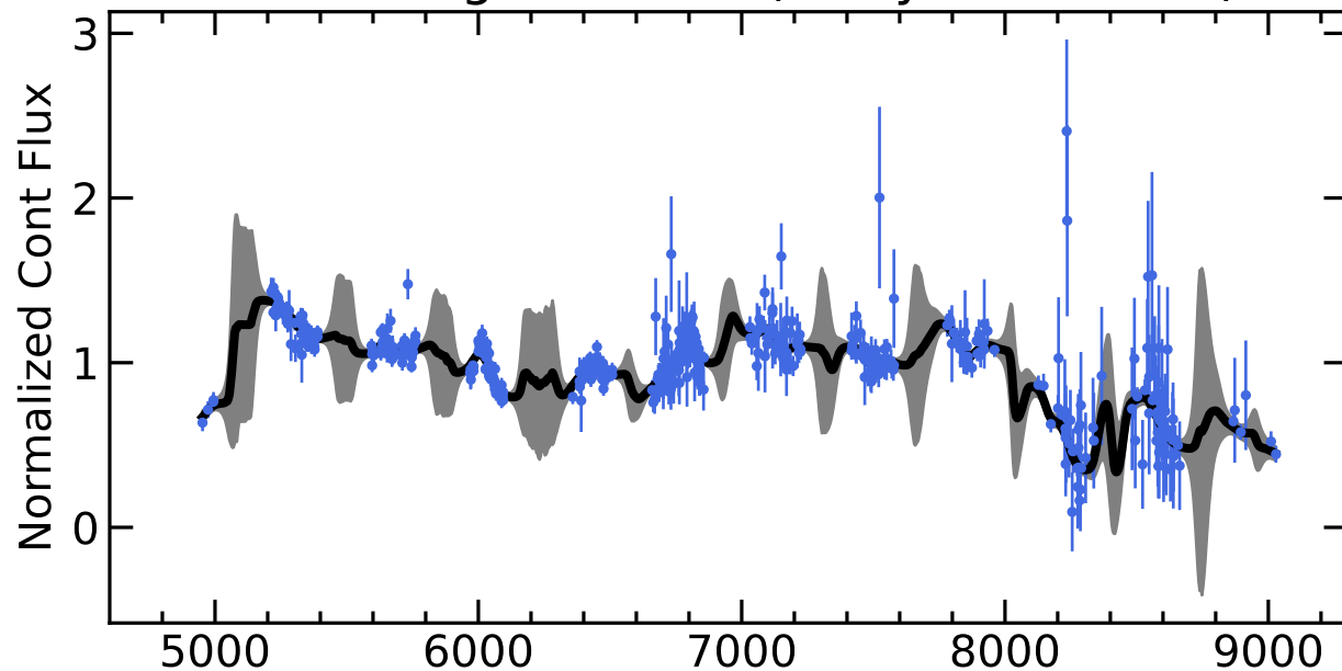
RM336 Light Curves (w/ PyROA model)
