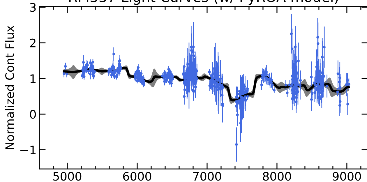
RM337 Light Curves (w/ PyROA model)
