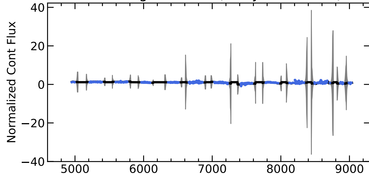
RM337 Light Curves (w/ PyROA model)
