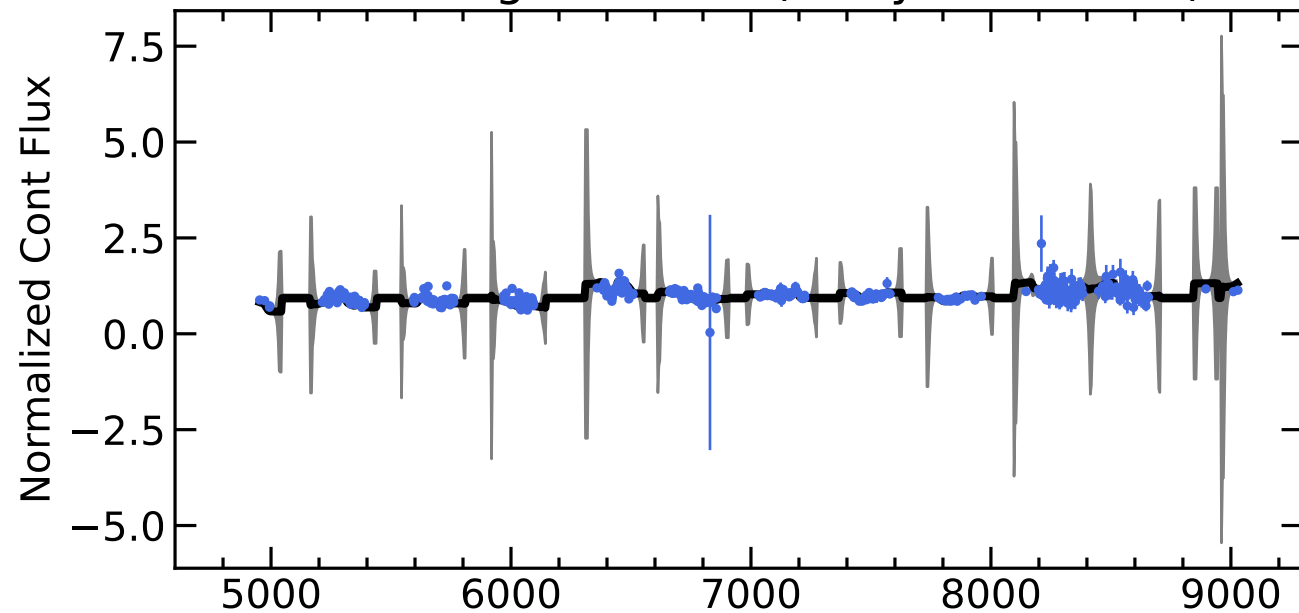
RM338 Light Curves (w/ PyROA model)
