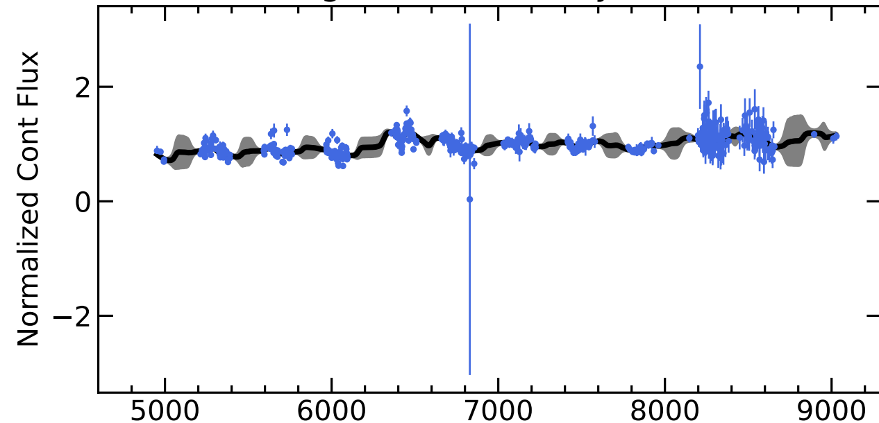
RM338 Light Curves (w/ PyROA model)
