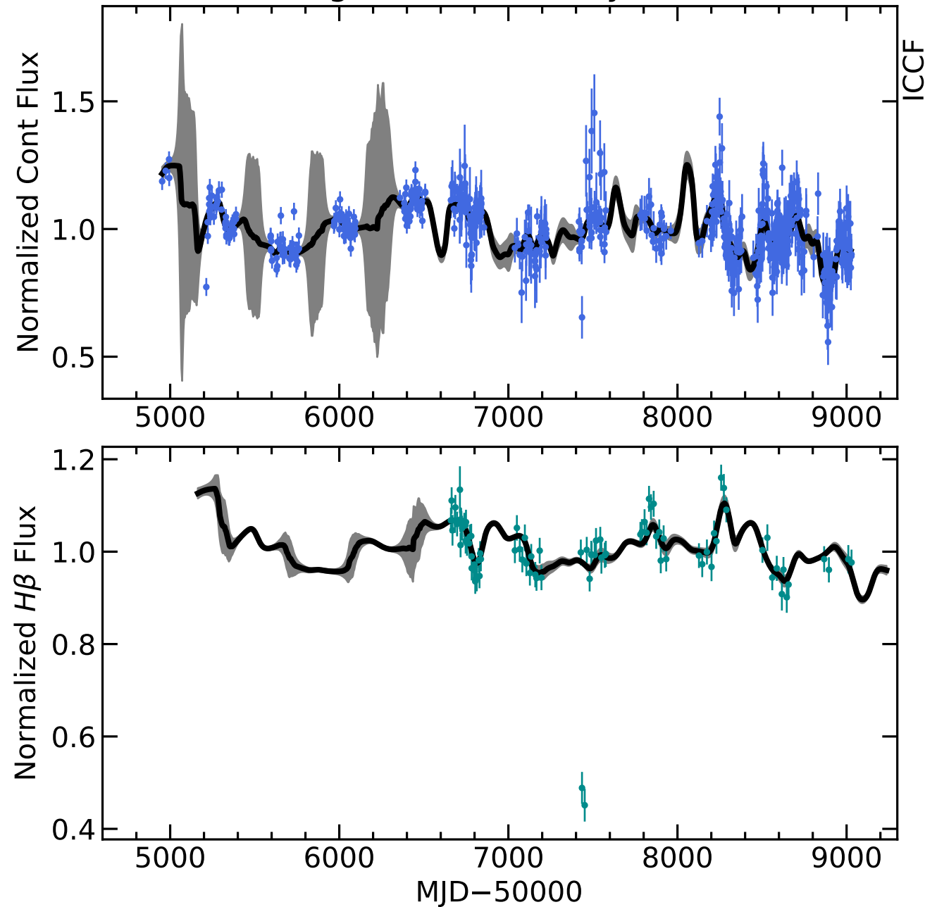
RM341 Light Curves (w/ PyROA model)
