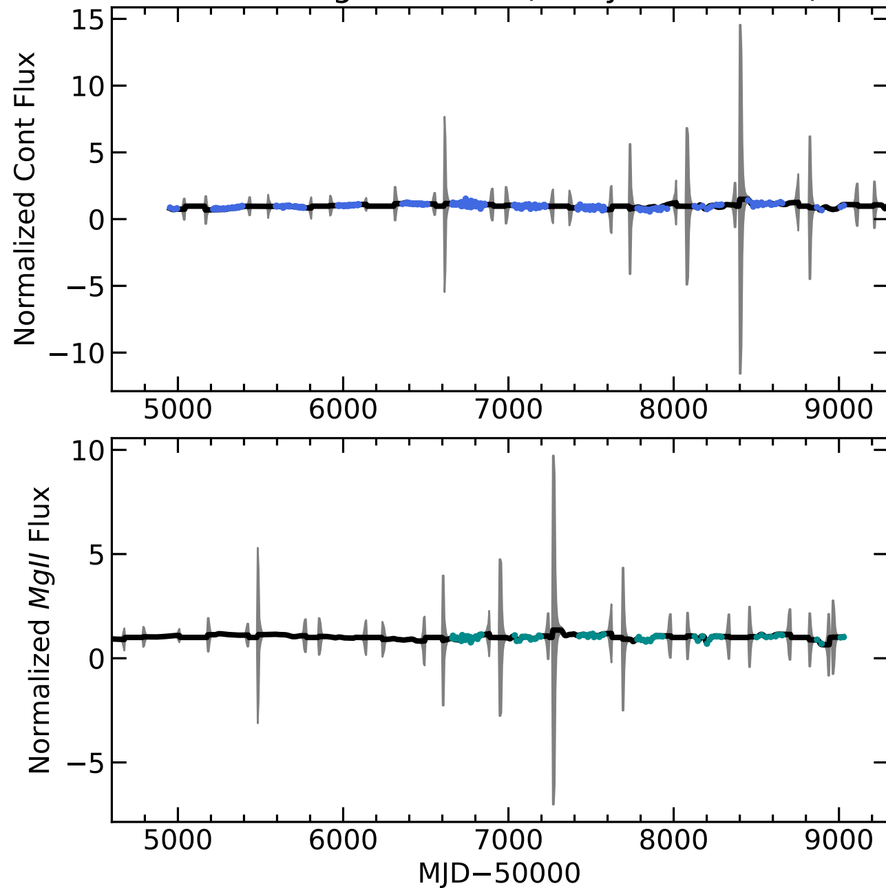
RM342 Light Curves (w/ PyROA model)
