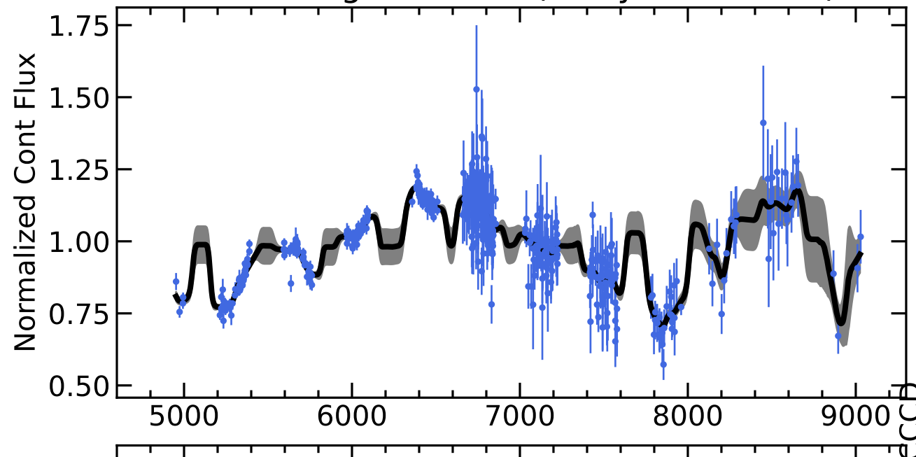
RM342 Light Curves (w/ PyROA model)
